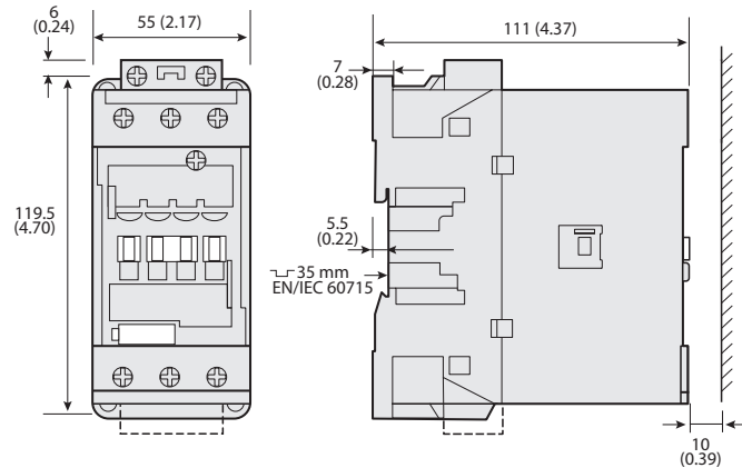
Figure 55 - 100-E40...100-E65 3-Pole Contactors
