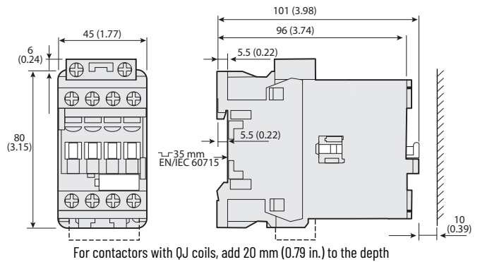
Figure 44 - 100-E26...100-E38 4-Pole Contactors with Low-consumption Coils
