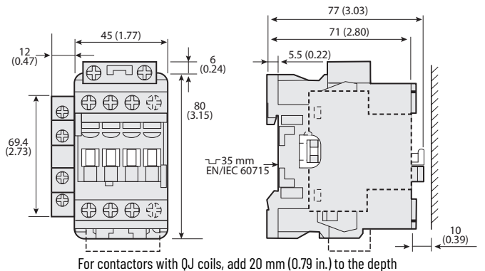
Figure 38 - 100-E09...100-E16 Contactors with Low-consumption Coils and Side-mounted Auxiliary Contact
