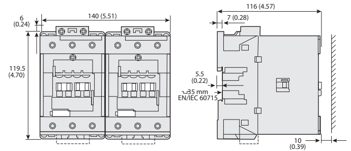
Figure 67 - 104-E80...104-E96 Reversing 3-Pole Contactors
