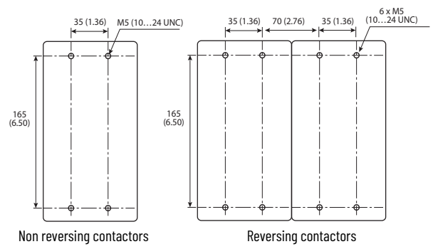
Figure 82 - 100-E265...100-E370 Contactors
