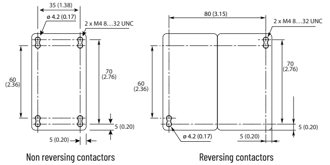
Figure 40 - Drilling Template for 9...16 A Contactors
