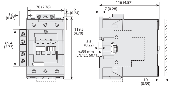
Figure 67 - 104-E80...104-E96 Reversing 3-Pole Contactors
