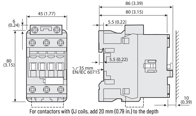
Figure 44 - 100-E26...100-E38 4-Pole Contactors with Low-consumption Coils
