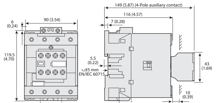
Figure 70 - 100-E80 4-Pole Contactors with Front-mounted Auxiliary Contact
