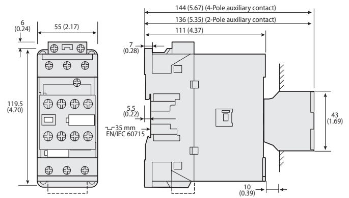
Figure 56 - 100-E40...100-E65 3-Pole Contactors with Front-mounted Auxiliary Contact
