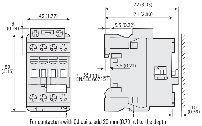
Figure 35 - 100-E09...100-E16 Contactors with Standard Coils and Front-mounted Auxiliary Contact
